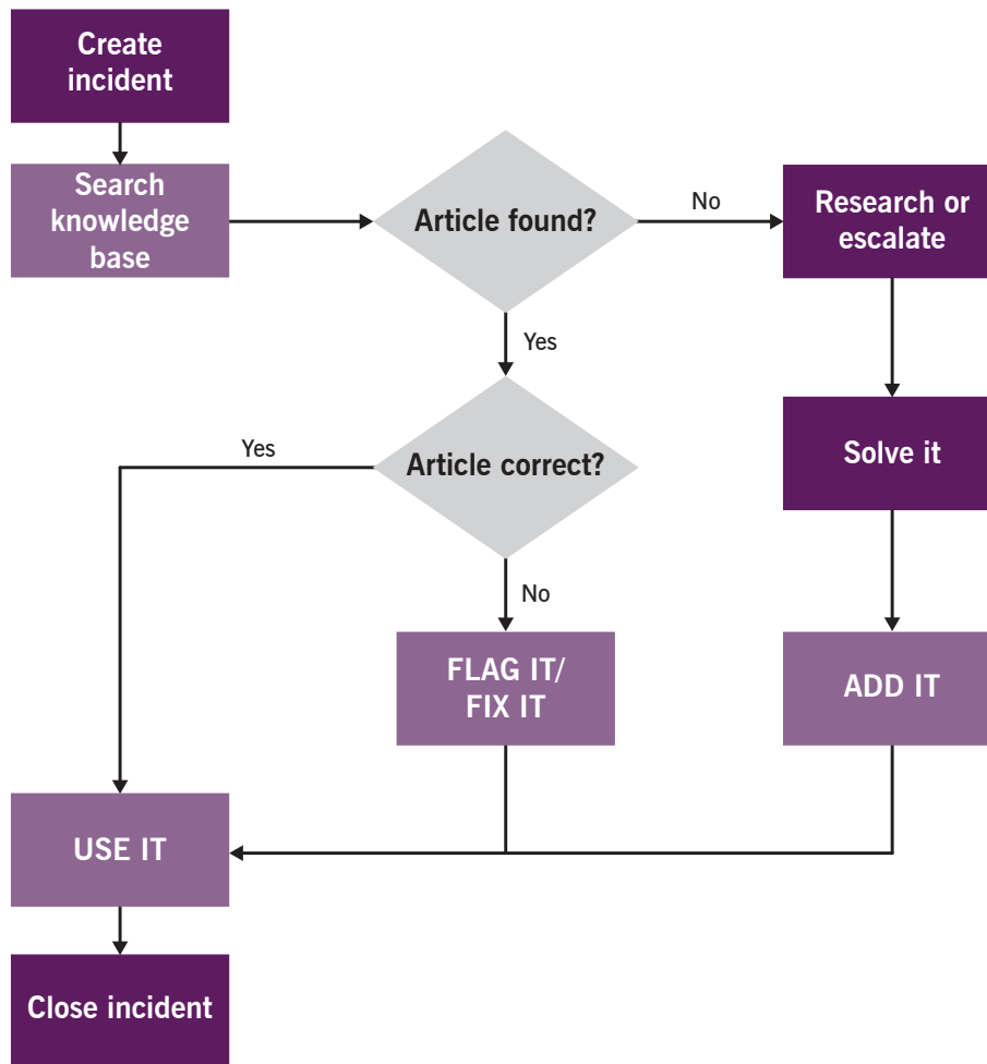
Figure 3 The UFFA workflow
